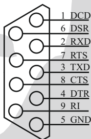
9-pin Cannon
