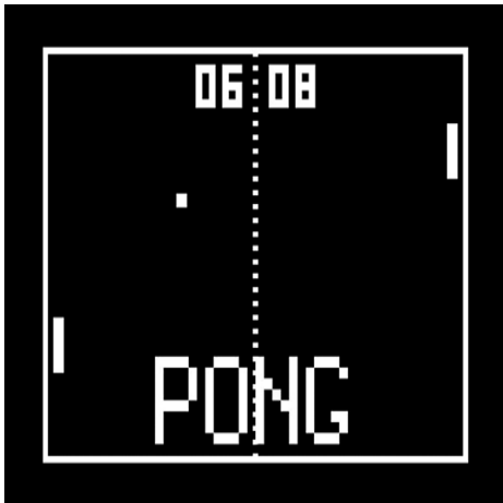
Pong
